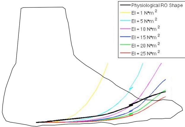
Figure 4. ANALYTICAL ROLLOVER SHAPES FOR CANTILEVER BEAM WITH UNIFORM CROSS SECTION AND VARYING BENDING STIFFNESS, EI
