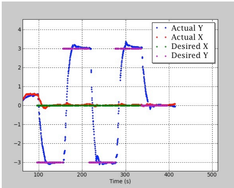
Figure 5 – Plot of actual X and Y coordinates in red and blue respectively compared to desired X and Y coordinates in green and purple. These tests were conducted in a controlled environment. This graph demonstrates centimeter level precision when hovering.
