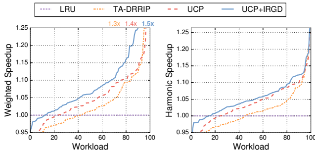
Figure 8: Weighted and harmonic speedup for 100 random mixes of SPEC CPU2006 apps. Our model enables partitioning of IRGD, improving performance over the state-of-the-art.
