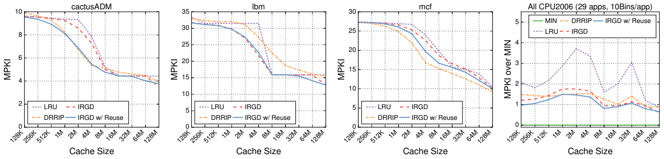
Figure 9: Misses per thousand instructions (MPKI) vs. cache size for (left) three applications and (right) all of SPEC CPU2006. Lower is better. Our model extends IRGD [39] to support reused/non-reused classification, making it outperform DRRIP on most applications and on gmean MPKI over all of SPEC CPU2006.
