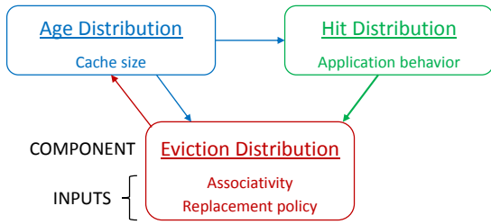
Figure 1: Our model consists of three interdependent probability distributions. Each distribution captures distinct model inputs. Arrows denote dependence, e.g. A \rightarrow B means “A depends on B”.
