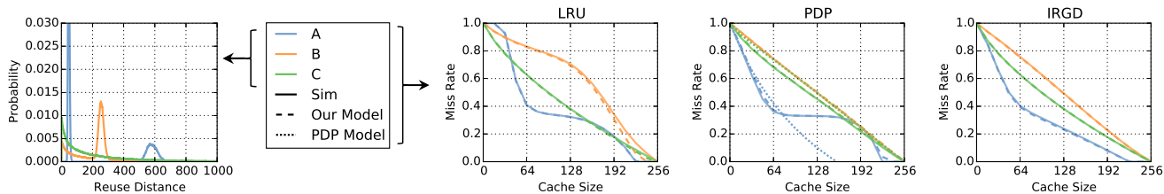
Figure 4: The cache model on three synthetically generated traces (A, B, C) driving small caches using LRU, PDP, and IRGD replacement. Simulation results are shown as solid lines; model predictions as dashed lines; PDP’s model as dotted lines.
