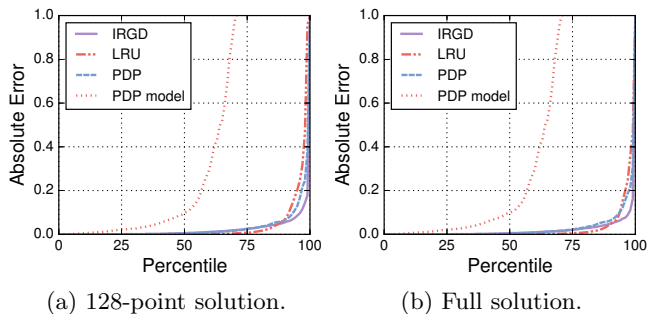
Figure 5: Model error distribution over 250 K-access intervals. Our model is accurate, while PDP’s model (dotted line) has large error.
