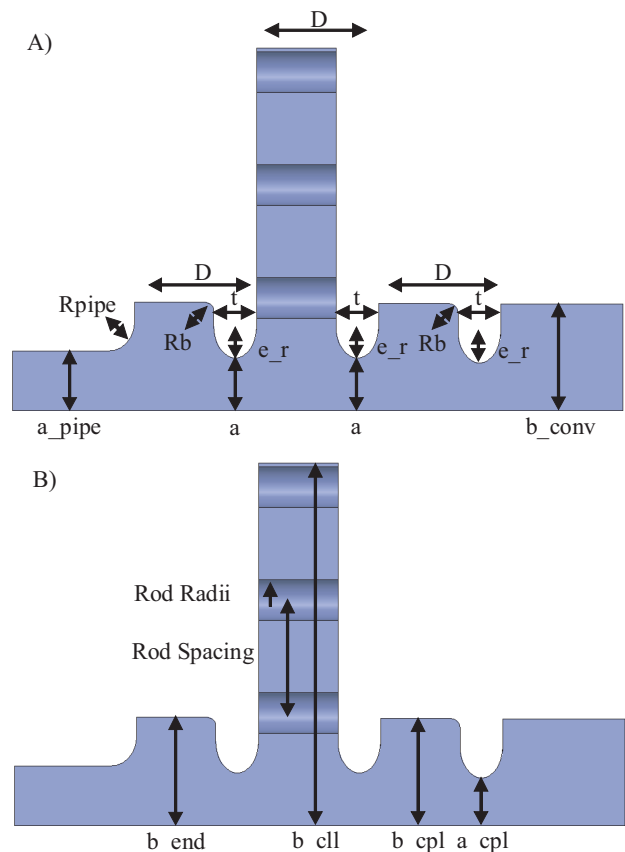
FIG. 5: Geometric parameters of PBG structure; A) fixed parameters, B) free tuning parameters, as shown in Table I and II, respectively.
