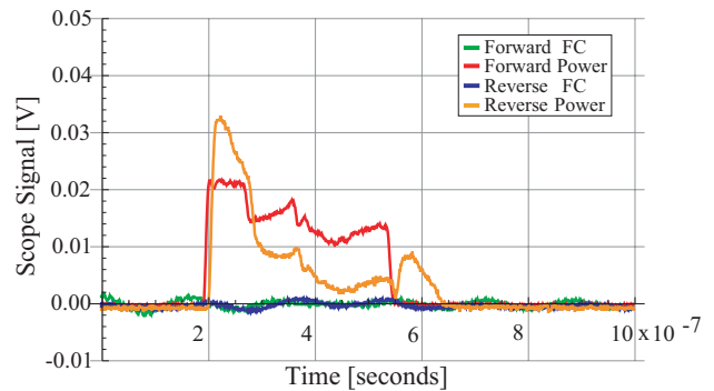
FIG. 14: Breakdown structure scope traces (uncalibrated) for non-breakdown event. Forward and reverse power in structure, forward and reverse Faraday cup signals. The forward power into the structure (from the peak power meter) was 5.0 MW for 170 ns for this shot.
