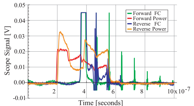
FIG. 15: Breakdown structure scope traces (uncalibrated) for breakdown event. Forward and reverse power in structure, forward and reverse Faraday cup signals. The forward power into the structure (from the peak power meter) was 5.0 MW for 170 ns for this shot.
