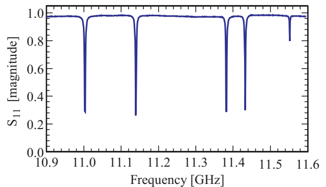
FIG. 11: Broad S_{11} measurement showing all observed resonances of the PBG structure and mode launcher. The operating mode is the second from the right, at 11.43 GHz
