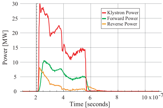
FIG. 13: Peak power meter trace for klystron signals: klystron output power, structure forward and reverse power traces. The forward power into the structure was 5.0 MW for 170 ns for this shot.
