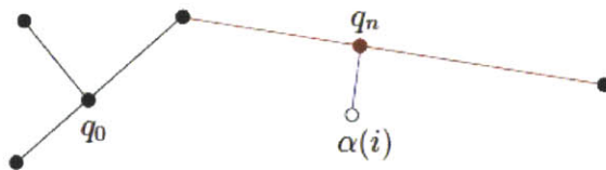
Figure 2.3: Extending an RDT Tree when the Closest Point is on an Edge [3]
