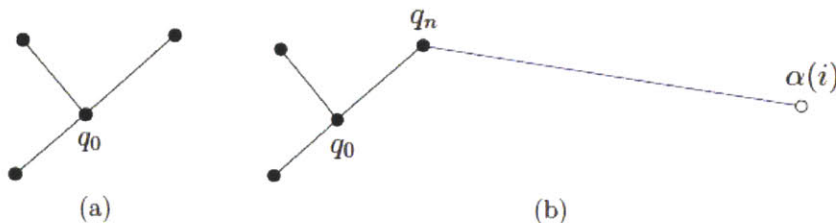
Figure 2.2: Extending an RDT Tree when the Closest Point is a Vertex [3]
