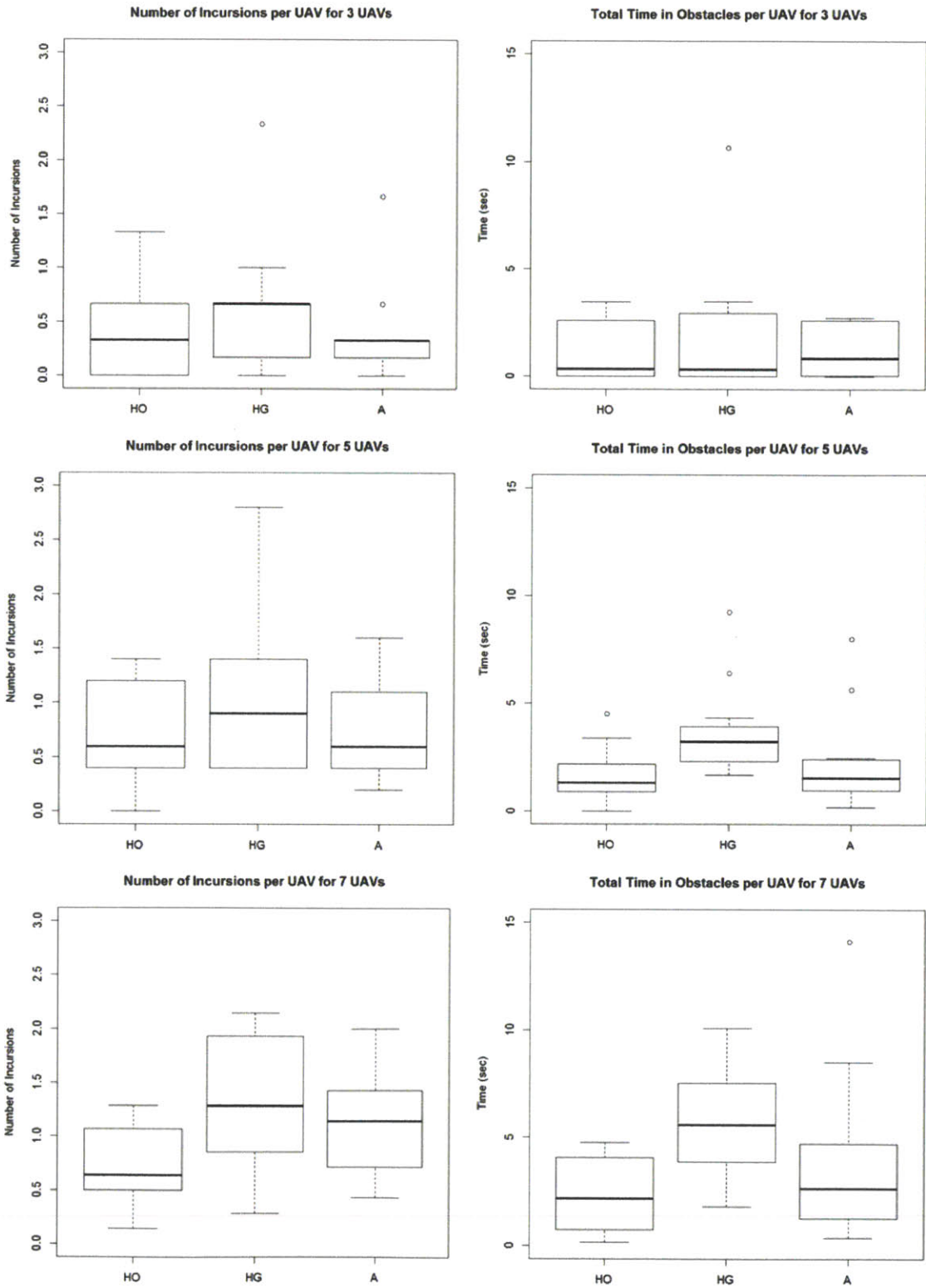
Figure 4.3: Number of Incursions per UAV and Total Time in Obstacles per UAV for 3, 5, and 7 UAVs
