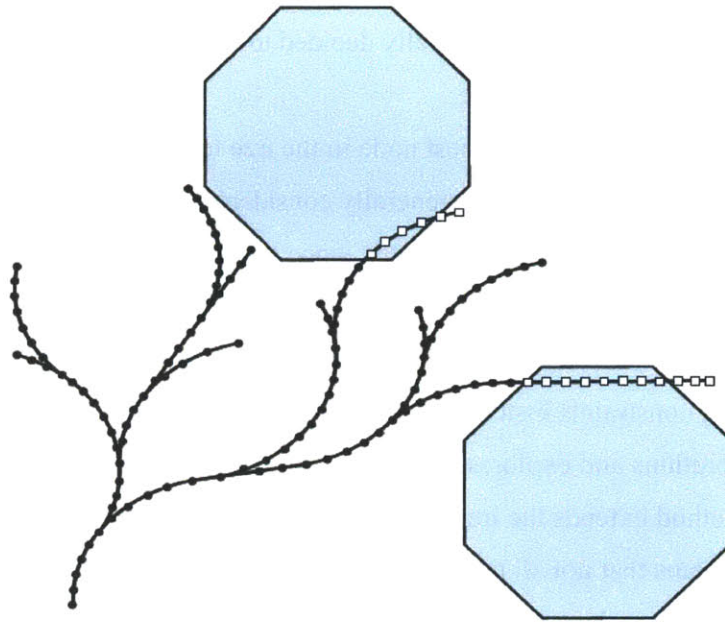
Figure 3.2: The RRT Algorithm [6]
