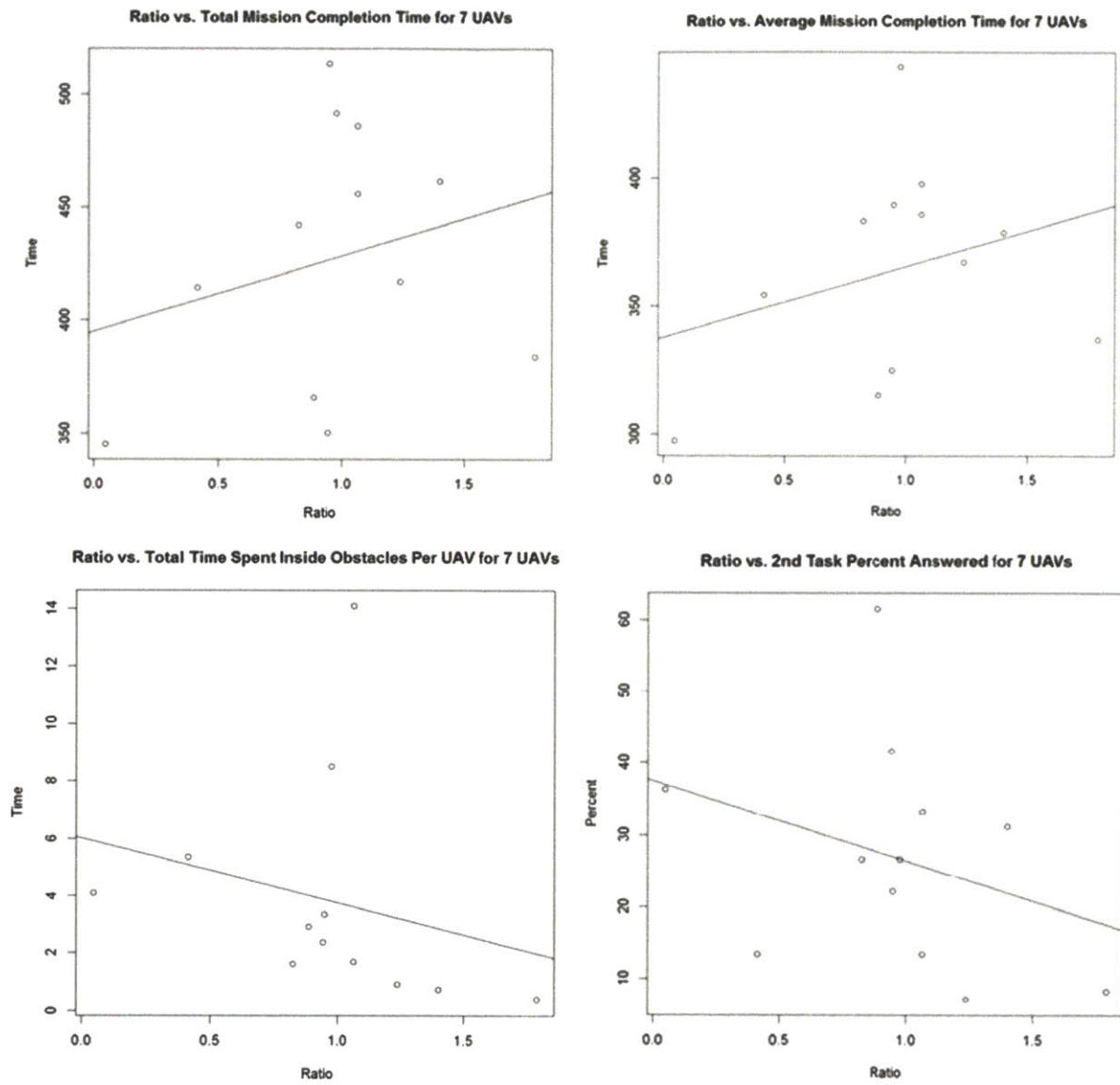
Figure F.2: Ratio of Waypoint Deletions to "Generate Path" Clicks vs. Various Metrics for 7 UAVs
