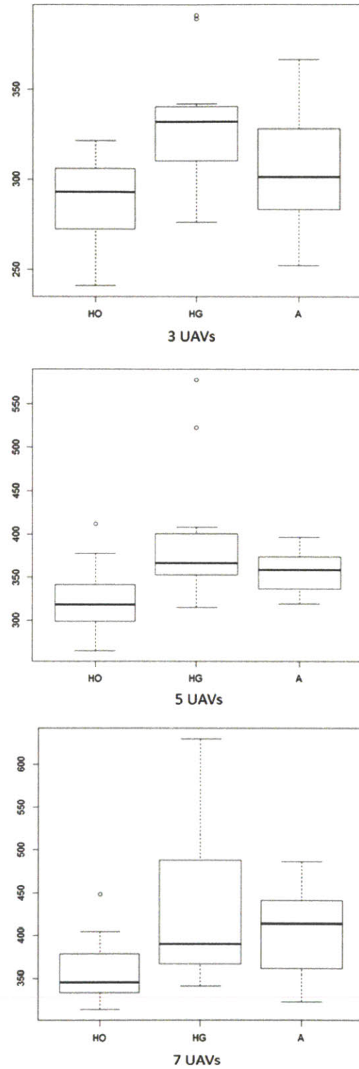
Figure 5.1: Total Mission Completion Times When the Last UAV is Ignored
