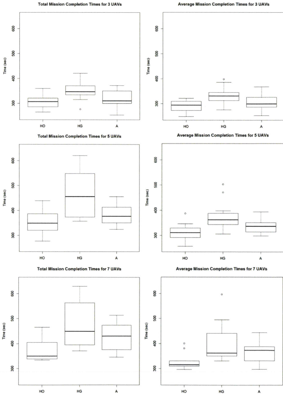
Figure 4.2: Total and Average Mission Completion Times for 3, 5, and 7 UAVs
