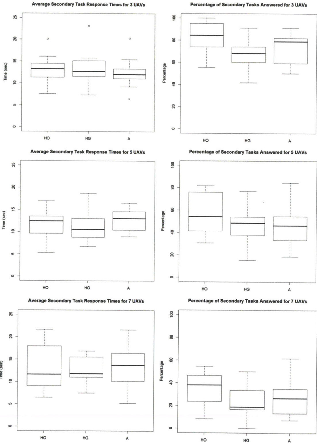
Figure 4.1: Secondary Task Response Times and Percentage of Secondary Tasks Answered for 3, 5, and 7 UAVs
