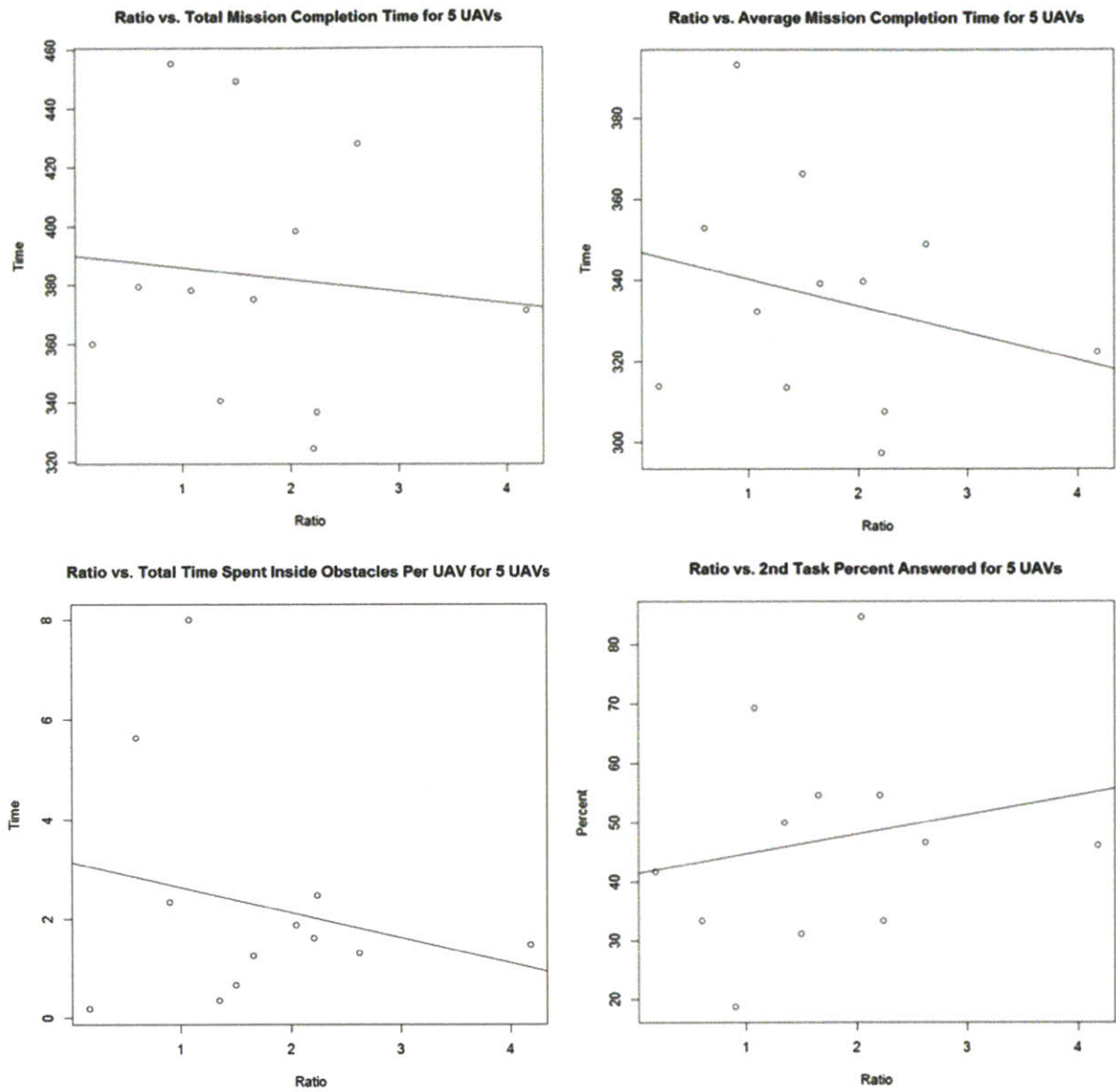
Figure F.3: Ratio of Waypoint Deletions to "Generate Path" Clicks vs. Various Metrics for 5 UAVs
