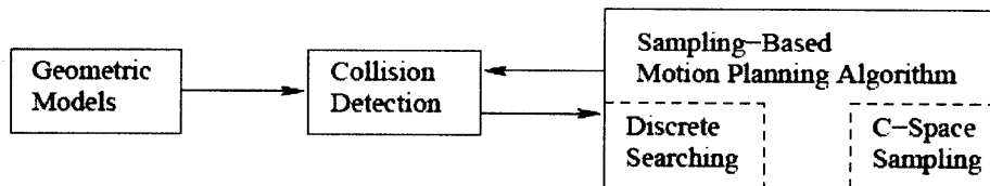
Figure 2.1: The Separation between Sampling-based Motion Planning Algorithms, Collision Detection, and the Geometric Models of the Environment [3]
