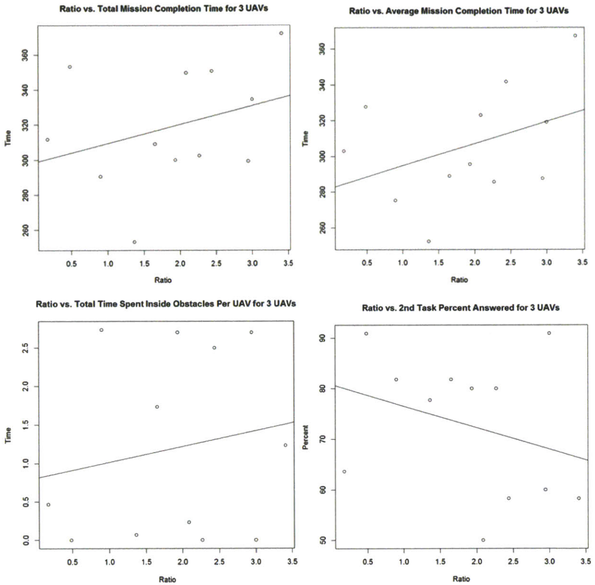
Figure F.1: Ratio of Waypoint Deletions to "Generate Path" Clicks vs. Various Metrics for 3 UAVs
