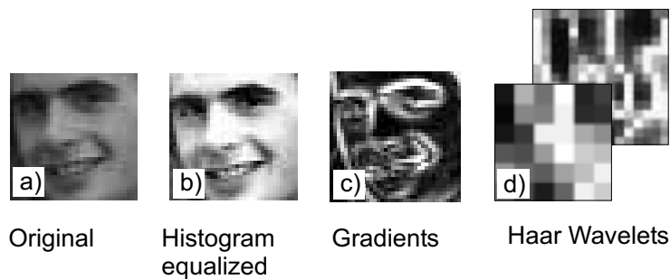
Figure 2: Examples of extracted features. The original gray image is shown in a), the histogram equalized image in b), the gray value gradients in c), and Haar wavelets generated by a single convolution mask in two different scales in d).
