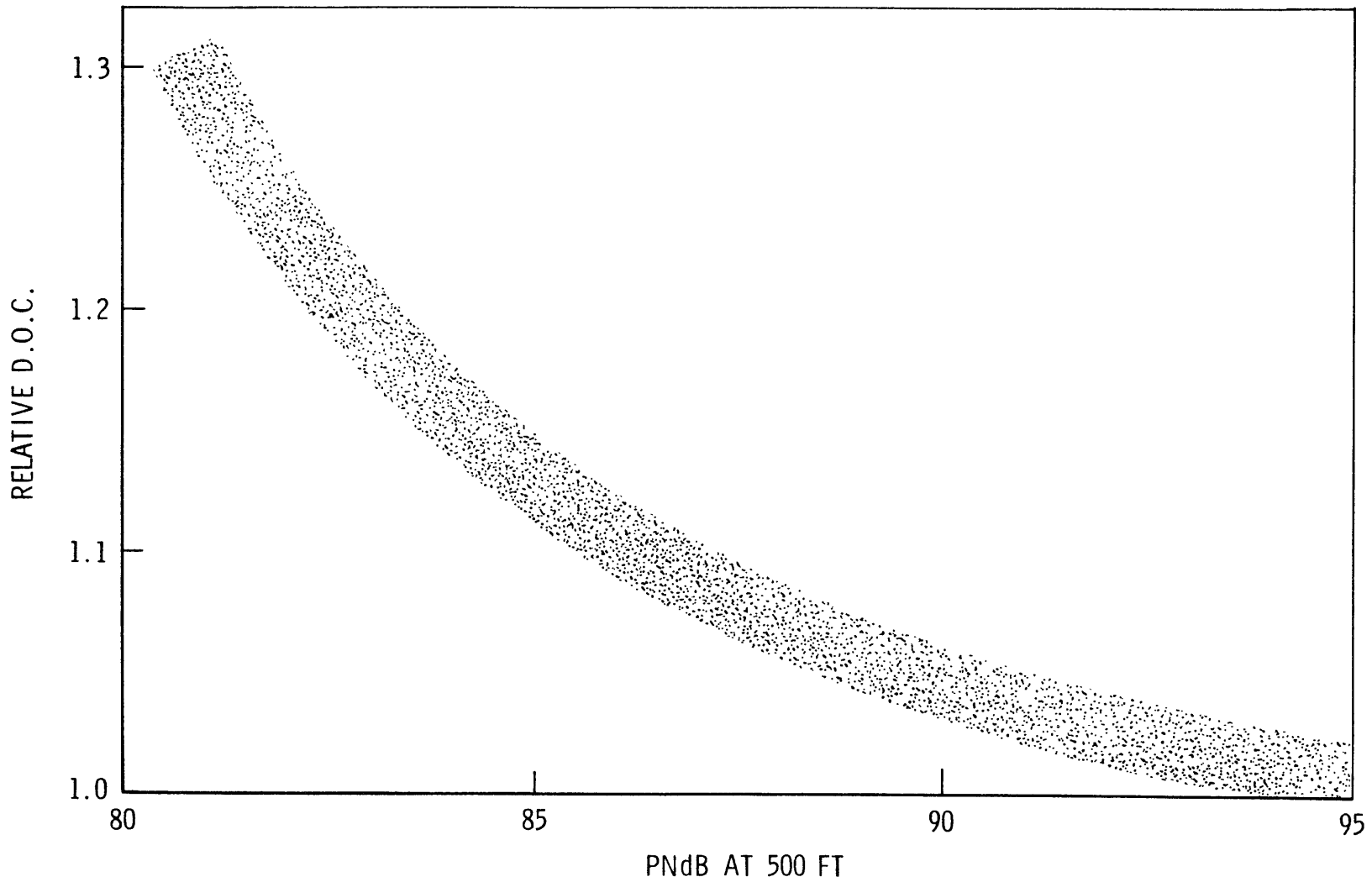
Fig. 3.12 Perceived Hover Noise vs Direct Operating Cost -- Future Helicopters
