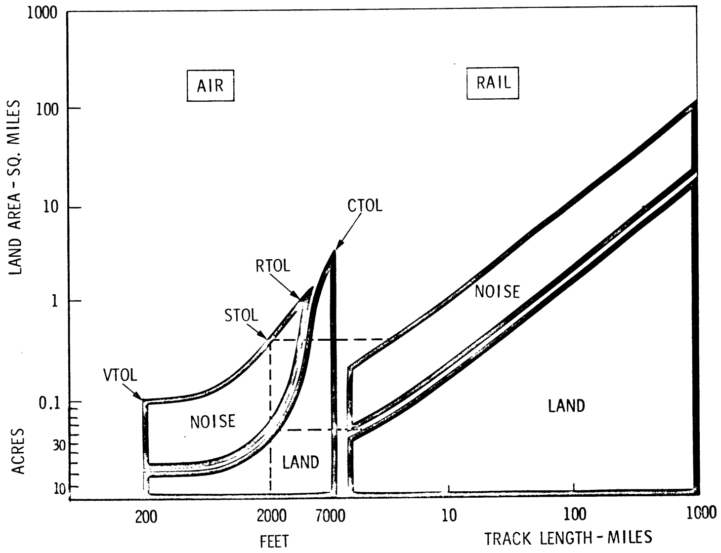
Fig. 2.2 Land and 90 PNdb Noise Areas -- 1980 Technology
