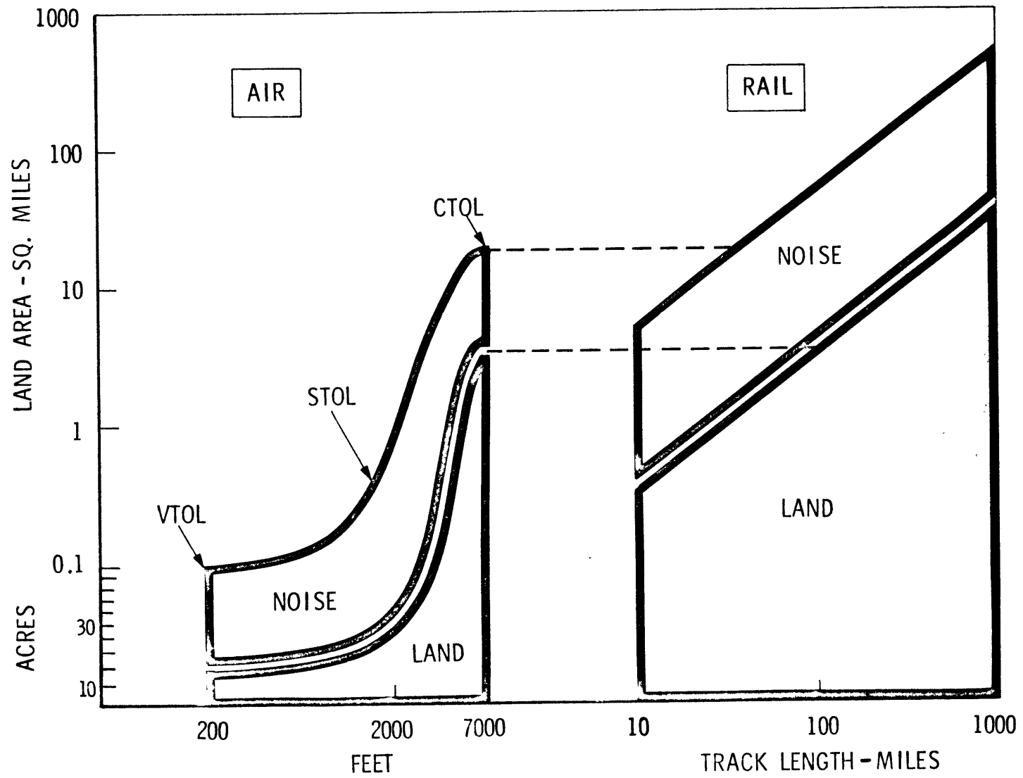
Fig. 2.1 Land and 90 PNdb Noise Areas-- 1960-70 Technology
