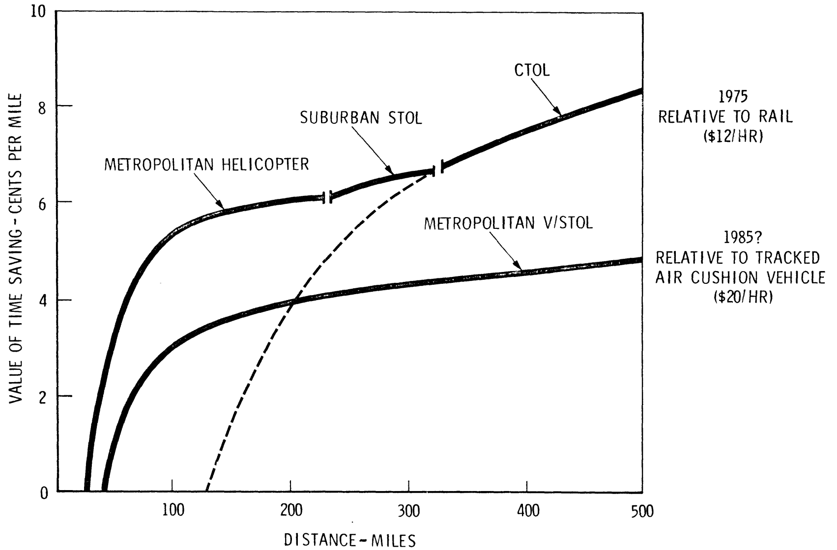
Fig. 2.7 Typical Values of Time Savings for Air: 1973 and 1985
