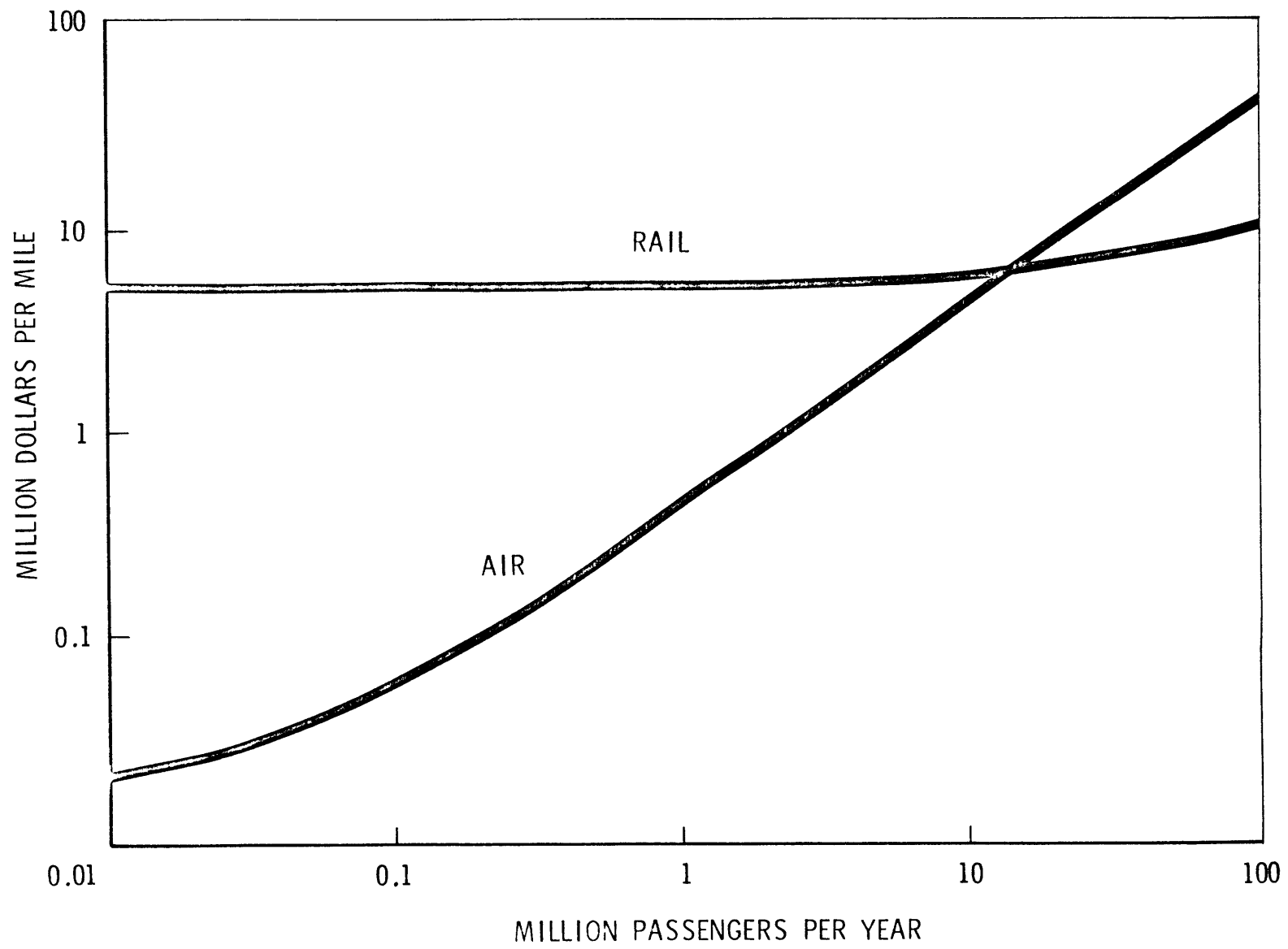
Fig. 2.3 Investment per Mile -- Rail and Air Systems
