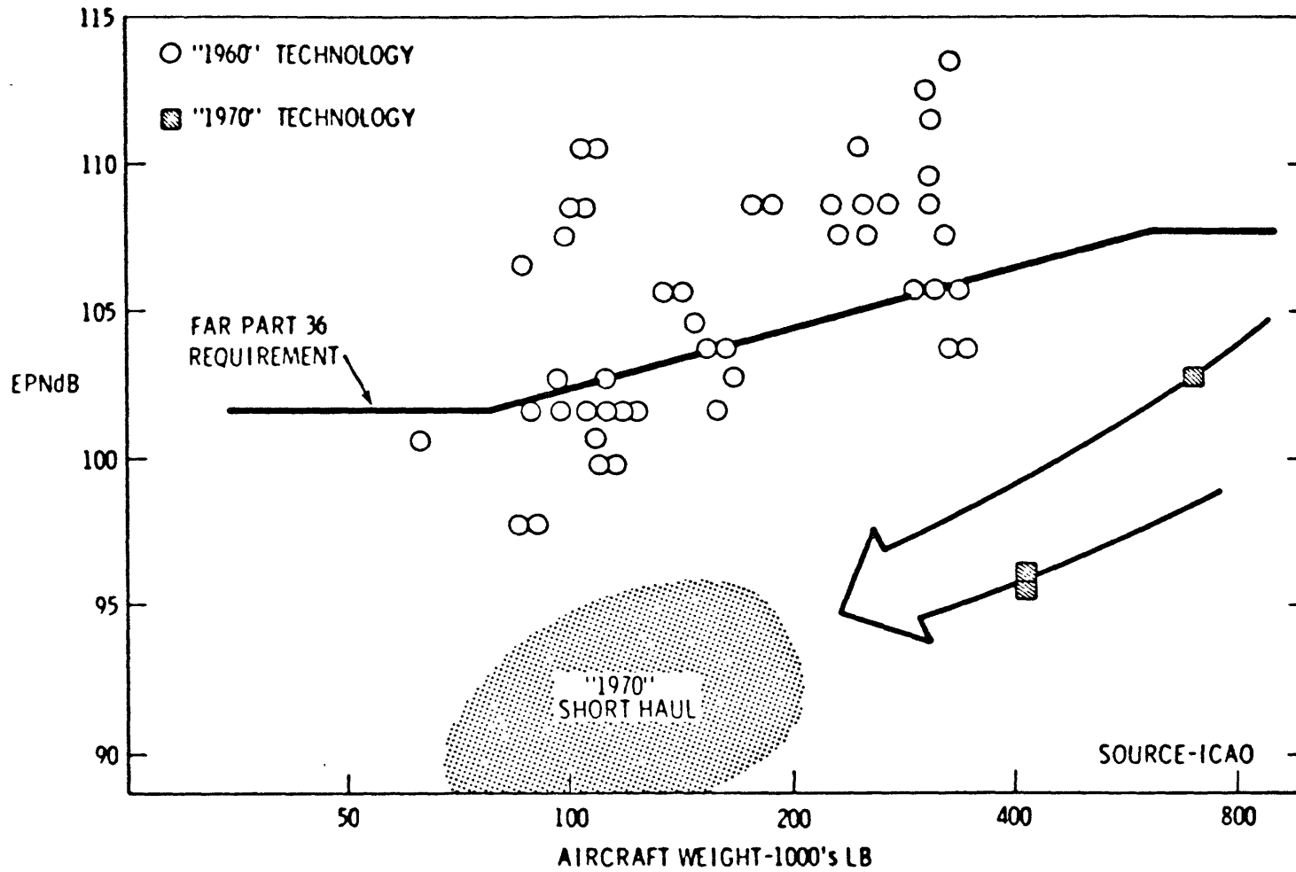
Fig. 3.5 Sideline Noise at Takeoff -- CTOL Transports
