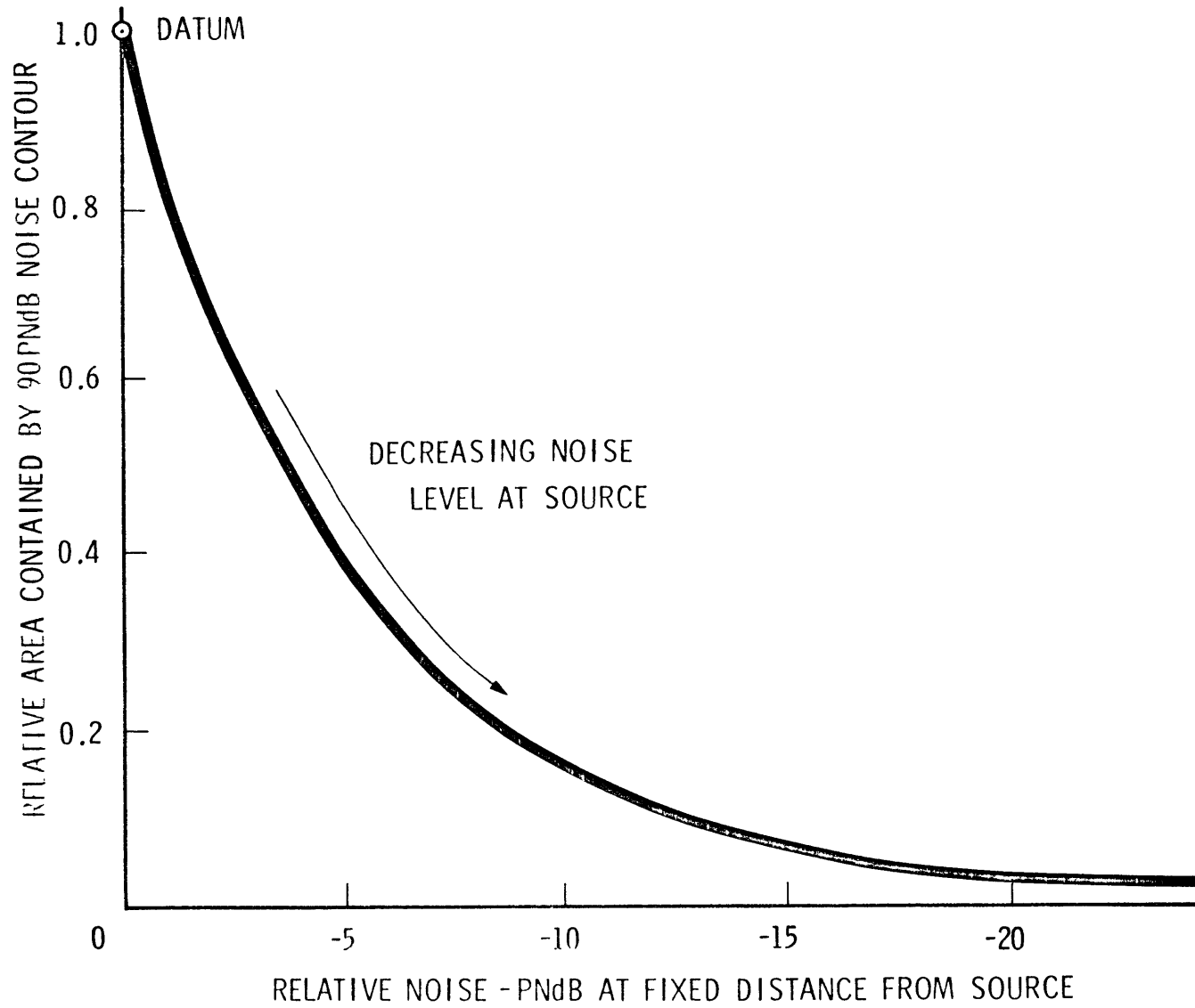
Fig. 3.7 Typical Variation of Footprint Area With Noise
