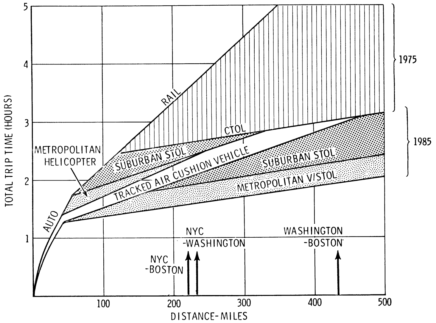
Fig. 2.6 Average Total Trip Times: NEC 1975 and 1985
