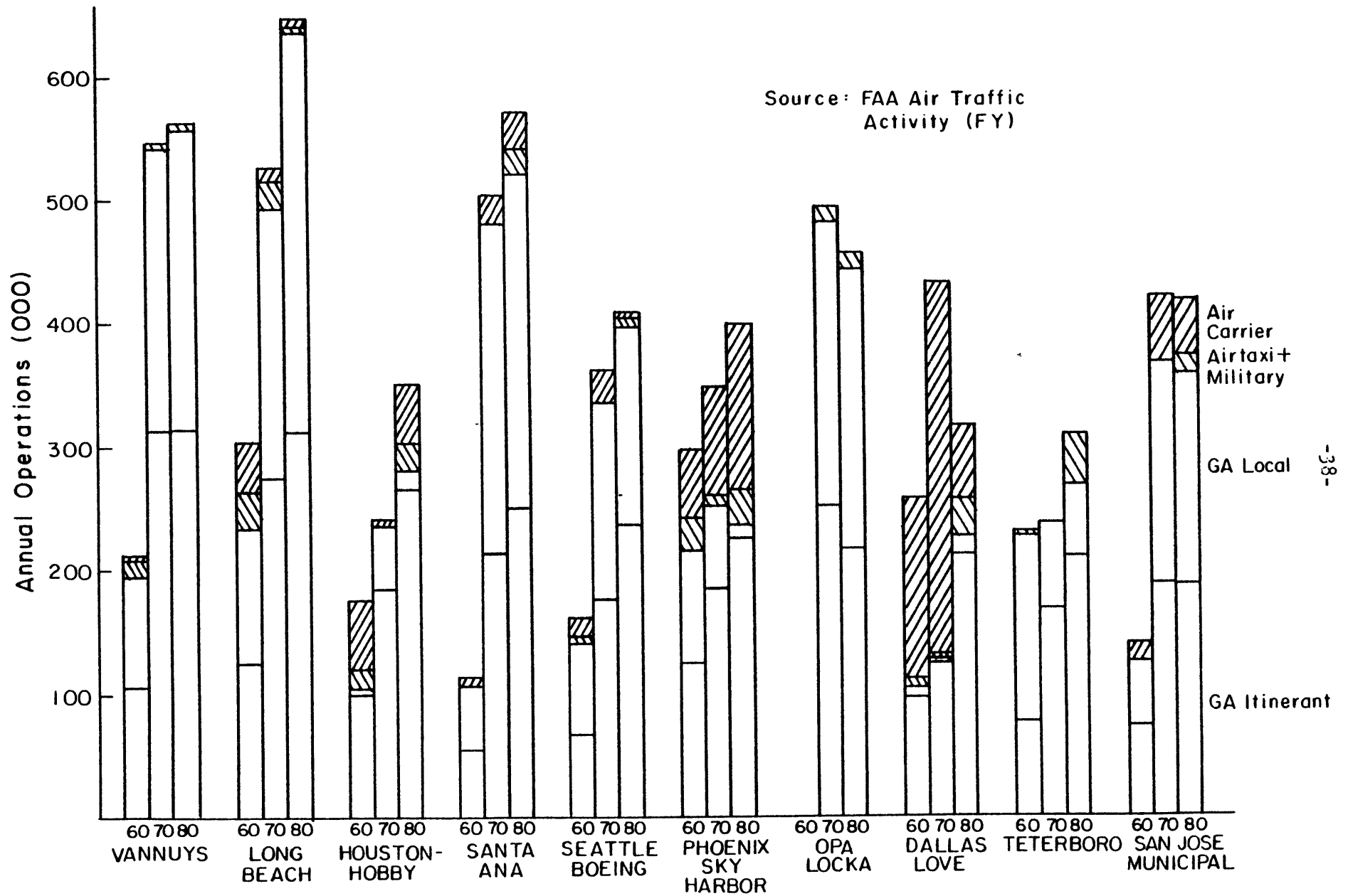
FIGURE 2.6 ANNUAL OPERATIONS AT TEN BUSIEST GA AIRPORTS
