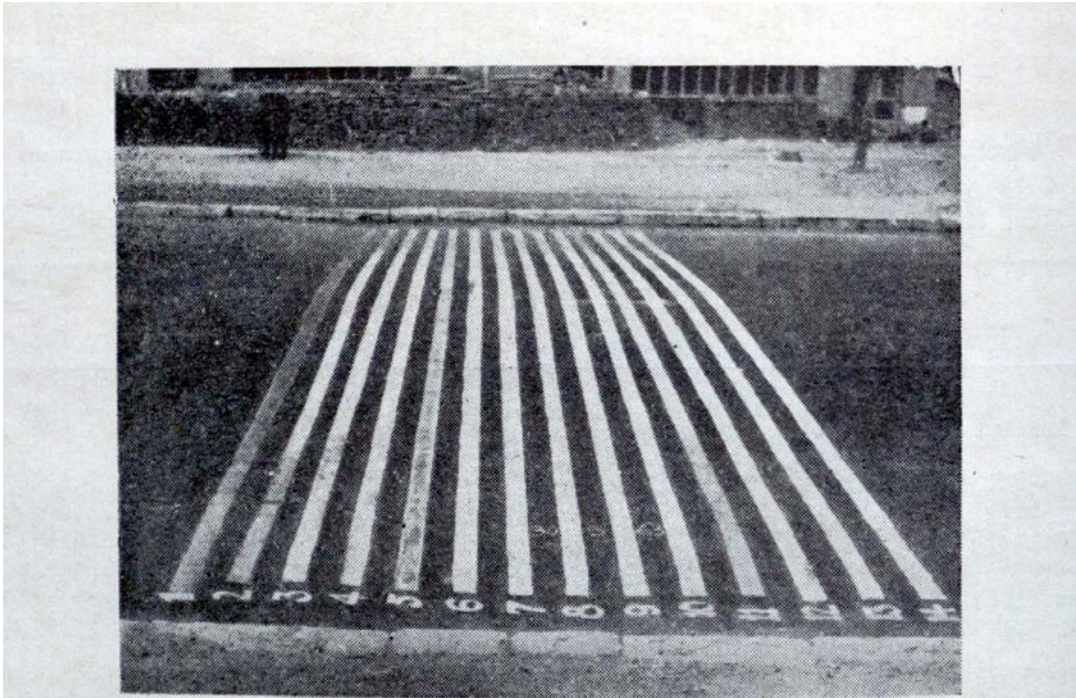
Fig. 25 (a) Transverse lines soon after painting
