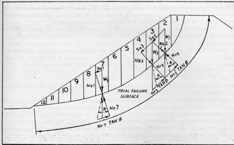
Fig. 12 Method of slices.
