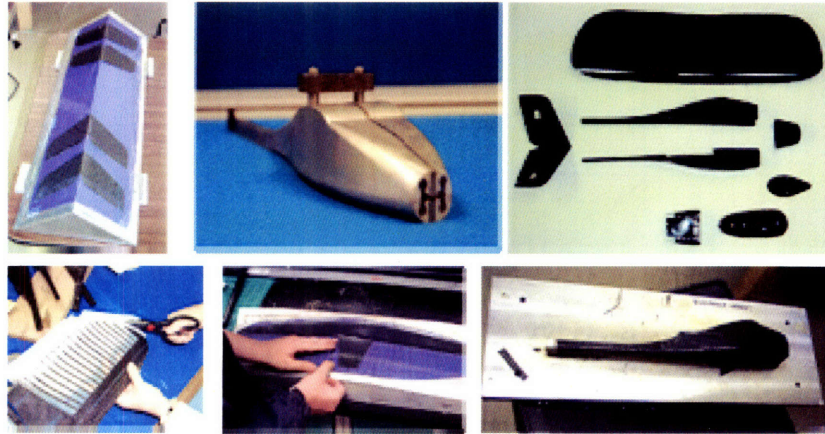
Figure 66: Manufacturing Components
