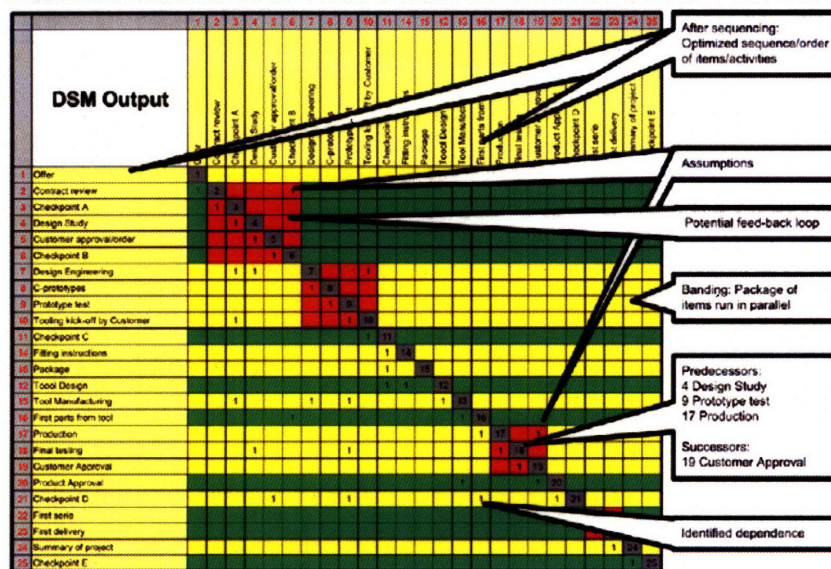
Figure 966: Activities DSM after Sequencing (Danilovic and Browning 2007)
