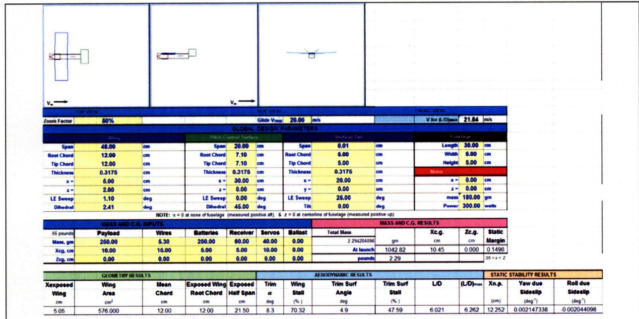
Figure 103: Screenshot of MAV Physics-based Model
