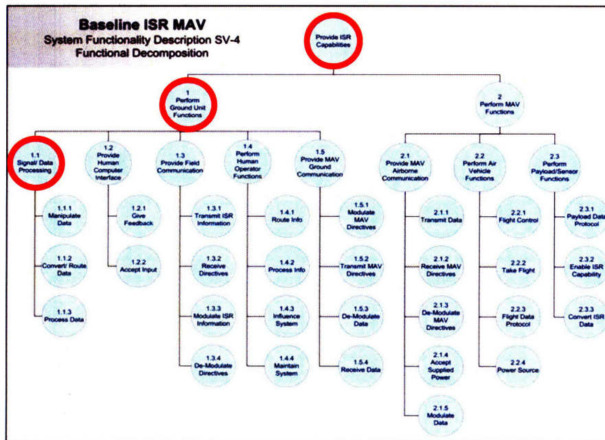
Figure 63: MAV Air Vehicle Functional Components represented by DoDAF SV-4 (Source Cooper, 2005)
