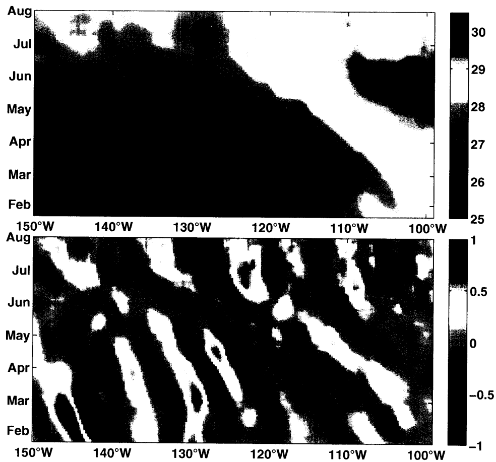
Figure 5-3: Upper panel: Longitude-time diagram of SST ( ^{\circ}\text{C} ) along 10.125^{\circ}\text{N} during 1998 from the TMI instrument. Lower panel: The same, except a 10^{\circ} longitude zonal running average has been removed to emphasize the mesoscale SST variability.
