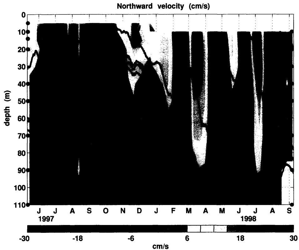
Figure 4-4: Depth-time plot of 10-day averaged meridional velocity at 10°N, 125°W. Current meter locations during the two deployments are indicated by blue dots on the left and right edges of the figure. The upper black line indicates the mixed layer depth (where the temperature is 0.1°C less than its surface value) and the lower three black lines are isotherms in the upper half of the thermocline (19, 22, and 24°C isotherms). Mixed-layer depth and isotherms are 10-day running averages.
