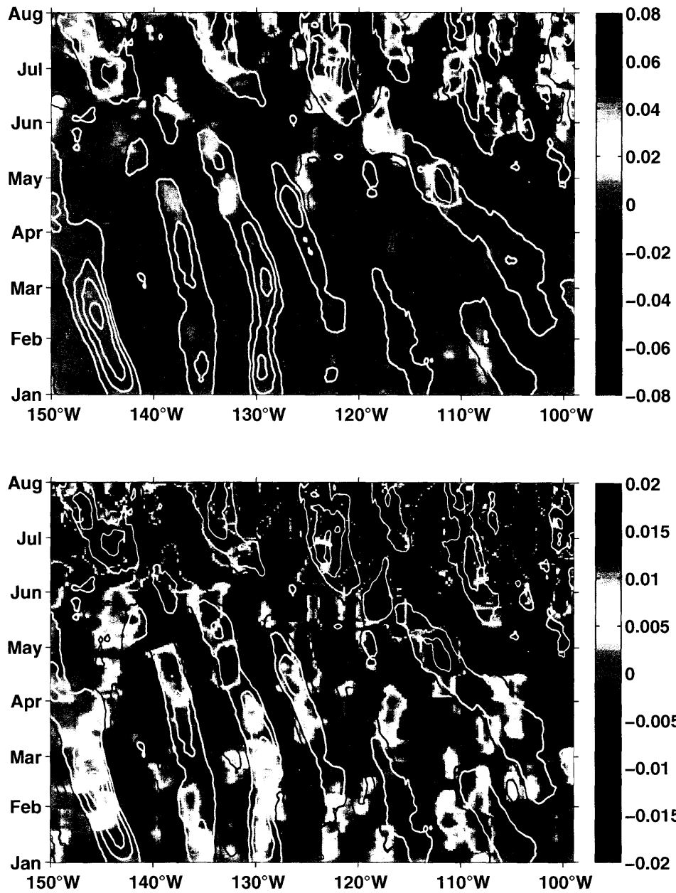
Figure 5-14: Both panels show filtered CLW (mm; colored) and filtered SST (white contours for warm anomalies, black contours for cool anomalies) along 10.125°N during 1998. The difference between the two panels is in the color scale. Note that CLW anomalies are about 10 times larger during the ITCZ season (June onward) than during the trade wind season (before April).
