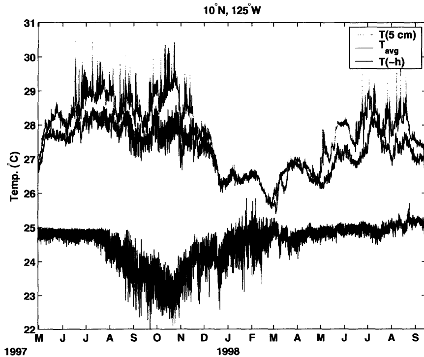
Figure 3-8: SST, T_a , and T_{-h} from the northern site. The integration was performed to the 1023 kg/m 3 isopycnal.
