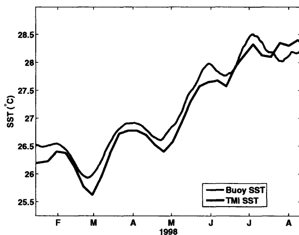
Figure 5-2: Comparison of SST from a buoy moored at 10°N, 125°W to SST at the same location from the TMI instrument. The buoy SST is a 21-day running average of hourly-average data; the TMI SST is a 21-day average of weekly-average data. The intraseasonal period band in the TMI data shows no clear evidence of contamination by aliasing of unresolved variability.
