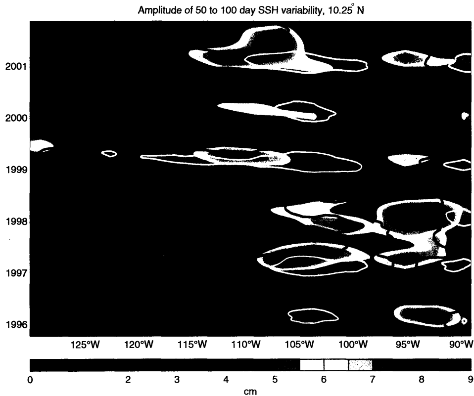
Figure 4-17: Amplitude of 50- to 100-day SSH signal along 10°N (color contours). Contours of low-frequency (125-day running-mean) zonal velocity are shown at -15 cm/s (black contours) and -25 cm/s (white contours).
