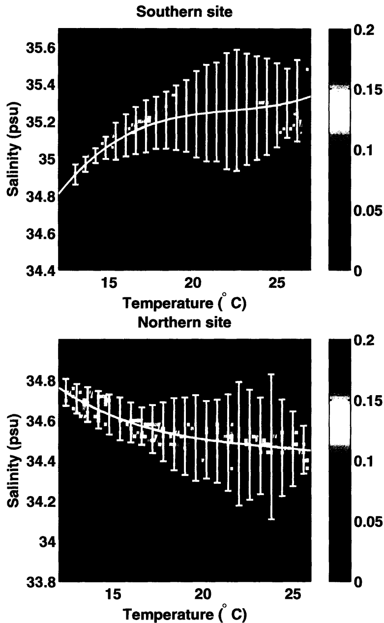
Figure 2-5: Colored fields: Fraction of the total salinity observations within each temperature class (0.2°C bins) accounted for by each salinity class (0.02 psu bins). In other words, the total number of observations in each T-S bin has been normalized by the total number of observations within each temperature bin. Upper panel: southern mooring site. Lower panel: northern mooring site. The white line shows the cubic fit described in the text, and the error bars encompass 85% of the salinity observations at within each temperature bin (see text for details). Isopycnals, computed for a pressure of 50 db, are overlaid at 0.25 kg/m 3 intervals (pink lines) to allow visual assessment of the error in density associated with errors in salinity inferred from the regression.
