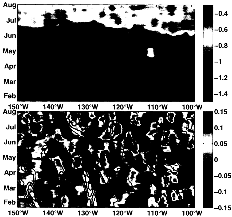
Figure 5-6: Upper panel: Longitude-time diagram of \log_{10} of cloud liquid water (CLW; in mm before taking the logarithm) along 10.125^{\circ}\text{N} during 1998. Lower panel: A zonally high-pass filtered version of the field in the upper panel (colored). Contours of positive mesoscale SST anomalies from Figure 5-3 are overlaid at 0.2^{\circ}\text{C} intervals, starting from zero.
