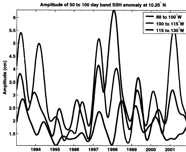
Figure 4-13: Estimated amplitude of 50- to 100-day variability in SSH anomaly at 10.25°N for three sub-regions of the eastern tropical Pacific Ocean. Edge effects potentially contaminate the results during about the first and last 140 days of each time series.
