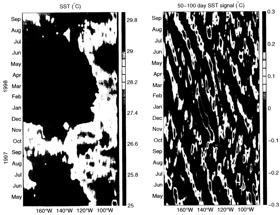
Figure 4-9: Left panel: AVHRR SST along 10.25°N. Right panel: 50- to 100-day SST signal along 9.75°N. In the right panel, a 15° longitude zonal running average was removed to filter SST fluctuations of larger zonal scales. The mooring was located at 125°W. For reference, zonal scales of 5° and 10° longitude are marked in March 1998. The solid diagonal line indicates a westward speed of 10 cm/s.
