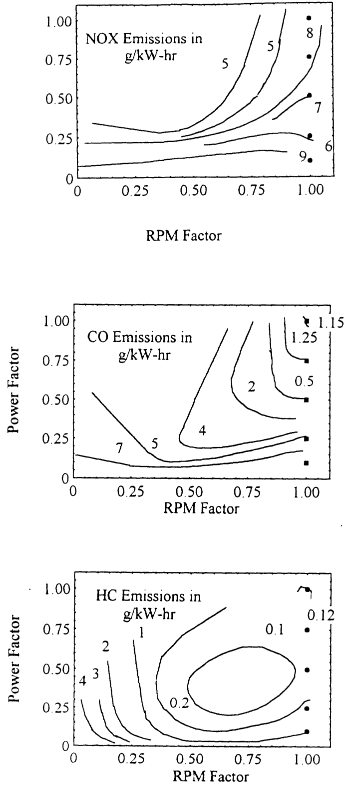
Figure C-9: ISO 8178 Duty Cycle D2
