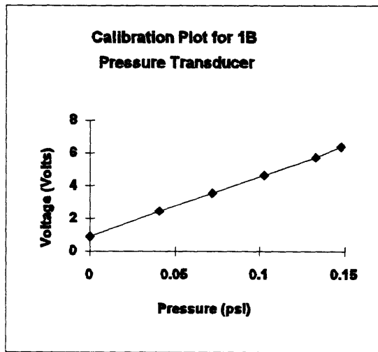
Figure D-12 : Pressure Transducer Calibration Curve
