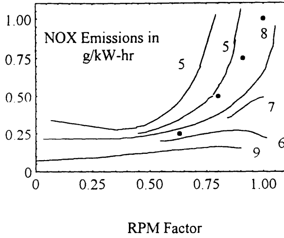
Figure C-5: ISO 8178 Duty Cycle E3
