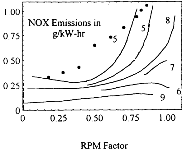
Figure C-1: MCM-1 Operating Profile (One Engine Per Shaft)
