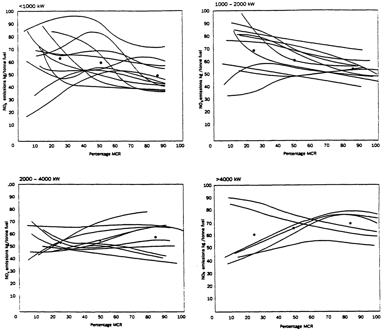
Figure 25: Lloyd's Register NO x Results 36
