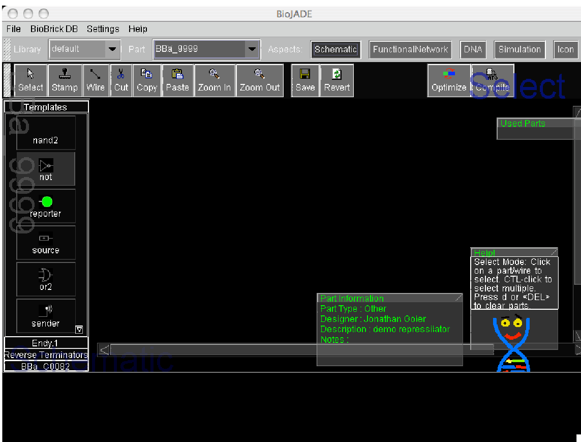
Figure 4.1: Schematic Design Mode. This figure shows the initial state of the schematic aspect. We have selected the not part prototype from the palette on the left.
