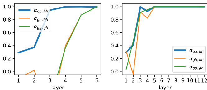
Figure 18: Alignment of different layers of a fully connected ReLU network at different layers (layer 0 is the input layer). Left : a 6-layer network. Right : a 12-layer network.
