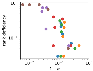
Figure 4: The rank deficiency and the backward \alpha_{gg, hh} in fully connected nets ( fc2 ). The rank of representation is strongly negatively correlated with \alpha . Here, every color is a different weight decay (from 10^{-6} to 10^{-4} ), and every point is a different layer in the net. The setting is the same as the fully connected net experiment.
