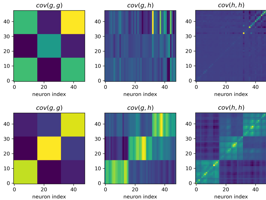
Figure 12: Representation covariance of the last convolutional block at initialization ( upper ) and end of training ( lower ).
