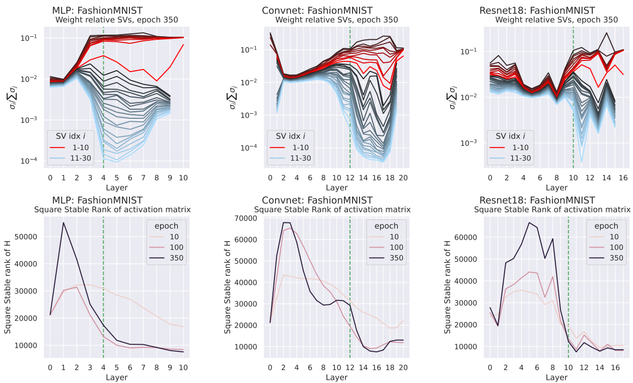
Figure 13: Estimates of Ranks of Weights and (Within Class) Features We see a low rank structure in the weights in collapsed layers, while previous layers are nearly full rank. This is also reflected in the stable rank of the features which first increases and then decreases in the collapsed layers.
