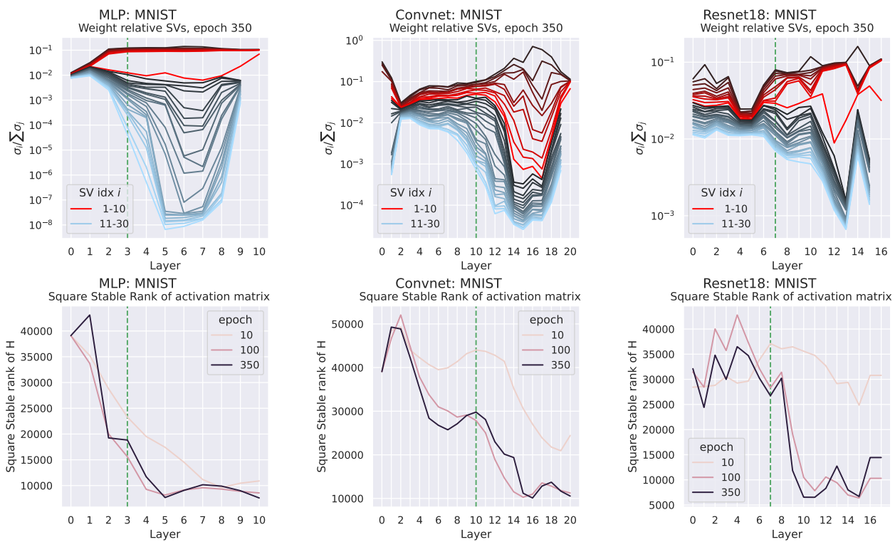
Figure 12: Estimates of Ranks of Weights and (Within Class) Features We see a low rank structure in the weights in collapsed layers, while previous layers are nearly full rank. This is also reflected in the stable rank of the features which first increases and then decreases in the collapsed layers.
