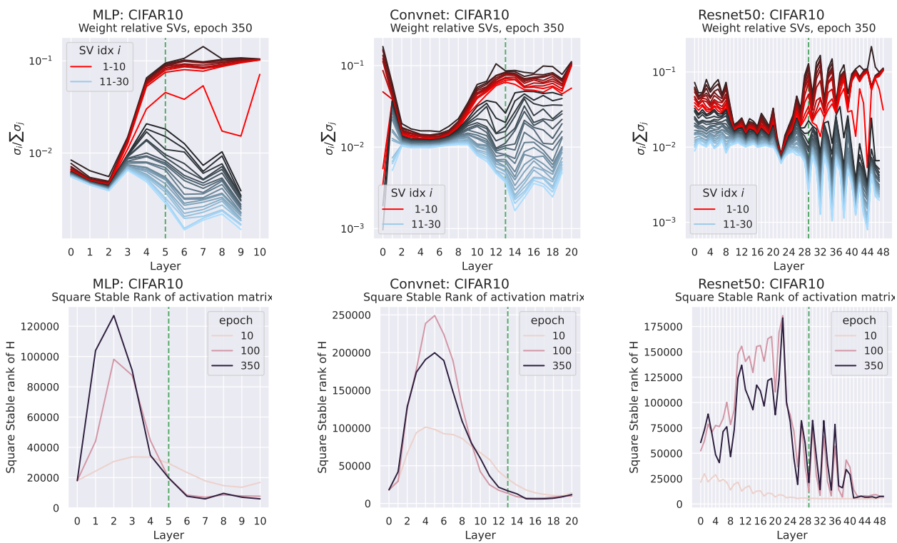
Figure 14: Estimates of Ranks of Weights and (Within Class) Features We see a low rank structure in the weights in collapsed layers, while previous layers are nearly full rank. This is also reflected in the stable rank of the features which first increases and then decreases in the collapsed layers.
