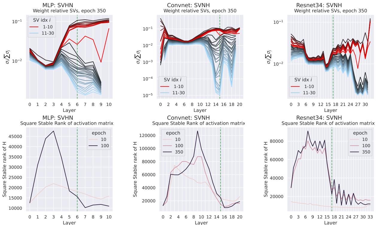
Figure 5: Estimates of Ranks of Weights and (Within Class) Features We see a low rank structure in the weights in collapsed layers, while previous layers are nearly full rank. This is also reflected in the stable rank of the features which first increases and then decreases in the collapsed layers.
