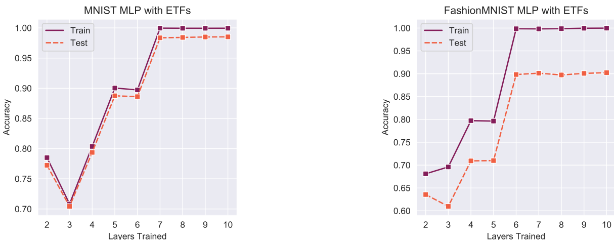
Figure 6: Comparison of performance of fixing collapsed layers to be ETFs We compare the accuracy achieved by fixing a certain number of layers to be simple ETFs. We see that fixing uncollapsed layers (lower than layer 6 in this instance) to be ETFs results in lower accuracy, while fixing collapsed layers (7 and above) does not hurt accuracy.
