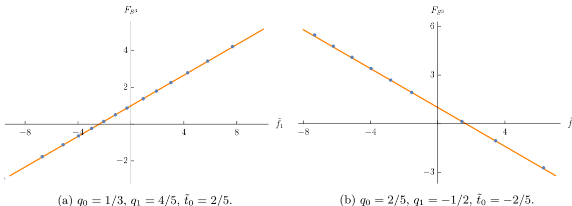
Figure 2. Value S_{\text{reg}} in a few examples. The blue points are values of S_{\text{reg}} computed numerically and the orange lines are the fit (3.34).
