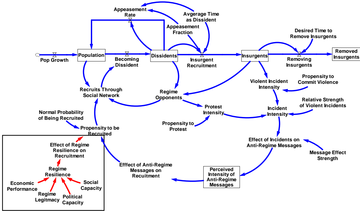
Figure 7: Regime Resilience
