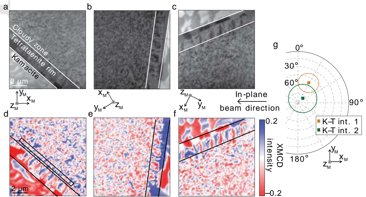
Fig. 1. (a–c) XPEEM images of one location along K–T interface 1 (supplementary Fig. S2). These images were obtained with right-circularly polarized X-rays at 707.2 eV (Fe L_3 absorption edge) for three different in-plane rotations of \sim 120^\circ of the sample. The grey scale quantifies the relative flux of electron captured in the optics. The in-plane azimuth of the beam is shown; it arrives at 30^\circ out of the plane of the image. (d–f) Corresponding XMCD contrast maps. A typical region-of-interest in the CZ is shown by a rectangle on panel (d). The tetrataenite rim is marked by the black lines. (g) Equal area projection showing the average relative direction of the paleofield estimated from the two K–T interfaces analyzed in Miles. Ellipses show the 95% confidence intervals accounting for the measurement uncertainty and counting statistical uncertainty. The reference frame refers to that of supplementary Fig. S2.
