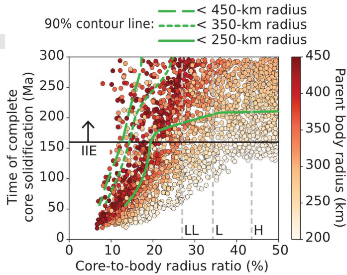
Fig. 3. Time of complete core solidification as a function of core-to-body radius ratio for partially- to fully-differentiated planetesimals with final radii between 200 and 450 km. Points represent the outcomes of cooling models conducted by Bryson et al. (2019b) for a wide range of accretion times and thickness of added chondritic material. The color bar indicates the final radius of the planetesimal. The time of solidification is an absolute upper limit, as it represents the time when the planetesimal reached the FeS eutectic temperature and all the latent heat of crystallization was extracted from the core. The horizontal black line shows the youngest time for complete solidification of the IIE parent body core recovered from the magnetic record of Miles. The three green lines mark the 90% contours for parent bodies with radius smaller than 250, 350 and 450 km. If we only consider parent bodies up to 250 km in radius, 90% of the simulations that produce the end of core solidification after 160 Ma after CAI formation have core-to-body radius ratios >19\% . This minimum ratio becomes 14% and 13% when including bodies up to 350 and 450 km in radius, respectively. The three gray vertical dashed lines show the core-to-body radius ratios calculated from the metal abundances of H, L and LL chondrites [ Krot et al., 2014 ] under the assumption that all the metal enters the core if bodies made of these meteorites were to differentiate.
