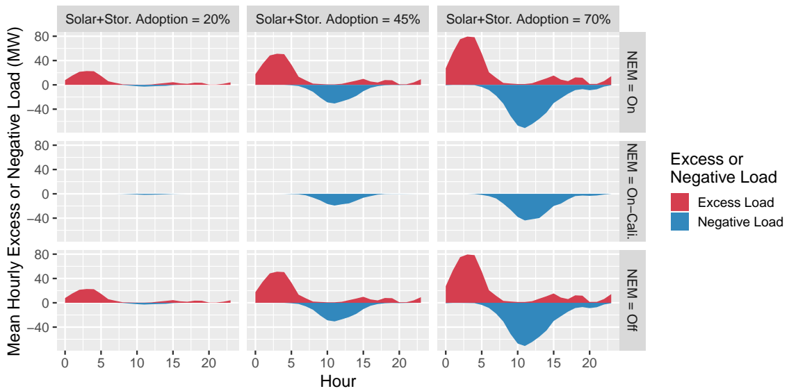
Figure 3-19: Excess load compared to original total load and negative load (or exports to the grid from customers) for all NEM regimes, different solar plus storage adoption levels and RTP-Efficient tariff.
