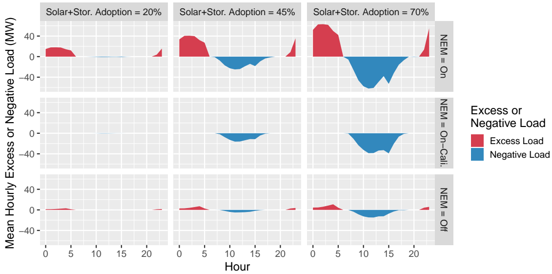
Figure 3-17: Excess load compared to original total load and negative load (or exports to the grid from customers) for all NEM regimes, different solar plus storage adoption levels and ToU tariff.
