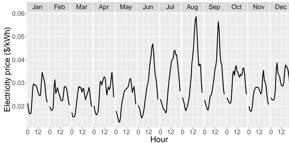
Figure 2-3: Real time pricing charges that include energy and capacity costs (hourly average).
