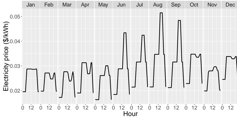
Figure 2-2: Time-of-use charges that include energy and capacity costs.
