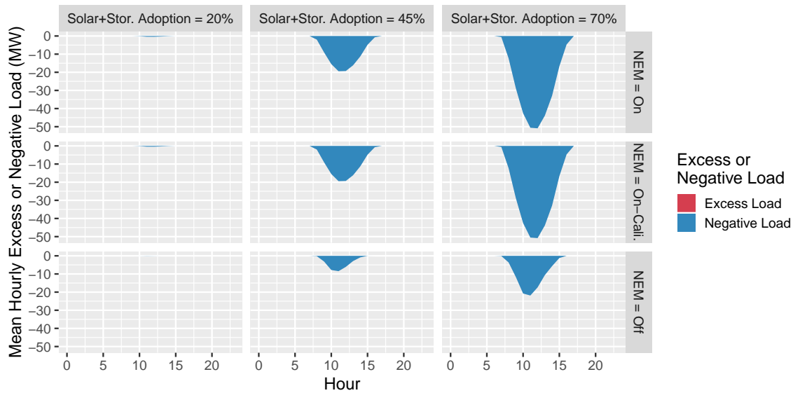
Figure 3-16: Excess load compared to original total load and negative load (or exports to the grid from customers) for all NEM regimes, different solar plus storage adoption levels and flat tariff.
