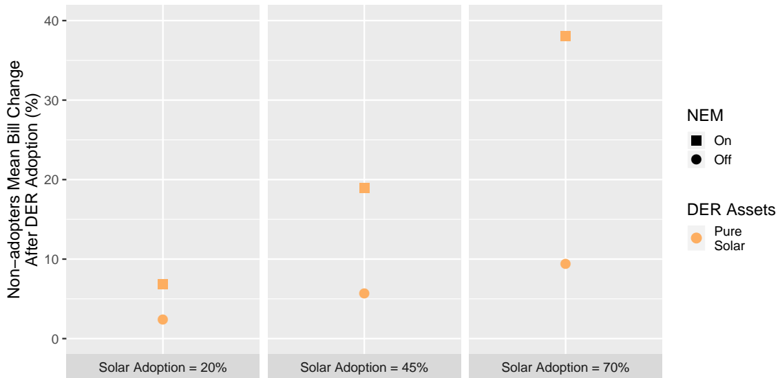
Figure 3-7: Mean bill change for non-adopters under different adoption levels (compared to the no adoption scenario), considering solar adoption alone and time-of-use tariffs.
