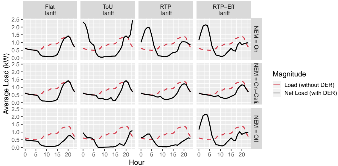
Figure 3-4: Hourly average of load and net load for a particular customer (same customer as figure 3-3).
