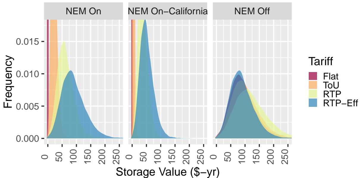
Figure 3-15: Marginal revenues (i.e., economic value) for solar adopters, triggered by installing storage under different NEM regimes and tariff designs.
