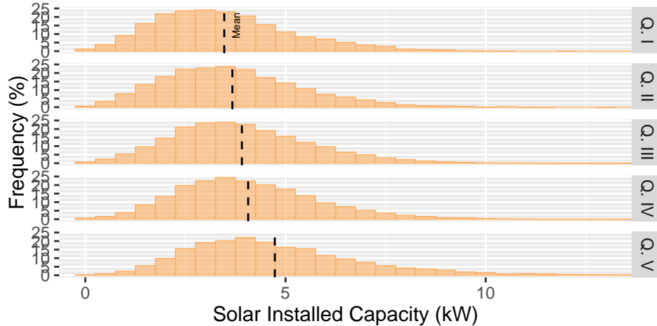
Figure 3-1: Solar installed capacity for each adopter customer in the 70% DER adoption scenario.
