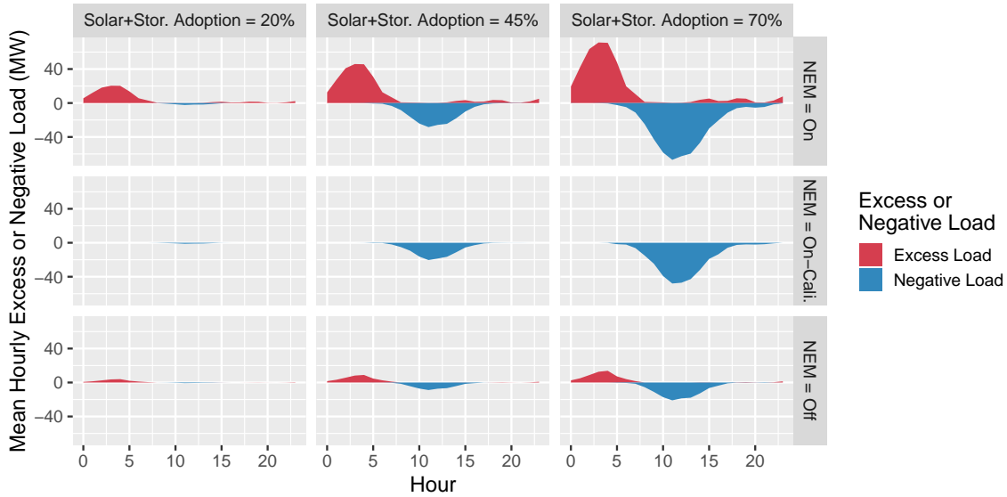
Figure 3-18: Excess load compared to original total load and negative load (or exports to the grid from customers) for all NEM regimes, different solar plus storage adoption levels and RTP tariff.
