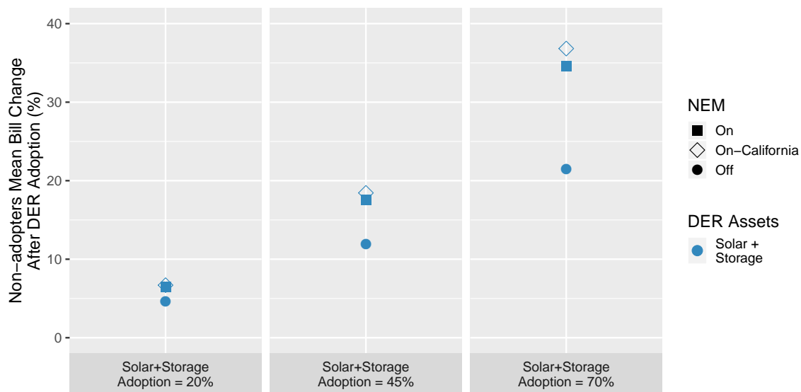
Figure 3-8: Mean bill change for non-adopters under different adoption levels (compared to the no adoption scenario), considering solar plus storage adoption alone and time-of-use tariffs.
