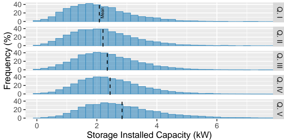
Figure 3-2: Storage installed capacity for each adopter customer in the 70% DER adoption scenario.
