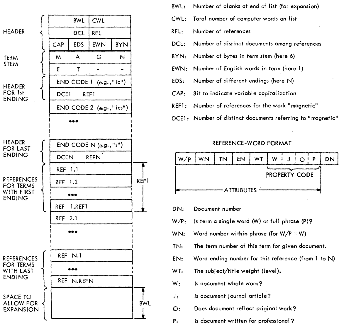
Fig. 13 Format for the Inverted File Subject-Term List
