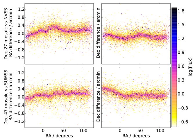
Figure 14.: Astrometric offsets (left: RA; right: Dec) for the 180 MHz mosaics, shown against RA (effectively, time of night). Top: Dec -27 mosaic, cross-matched against NVSS. Bottom: Dec -47 mosaic, cross-matched against SUMSS. The colour axis is the \log_{10} of the source flux density in Jy (as measured in the 180 MHz mosaic before amplitude calibration).
