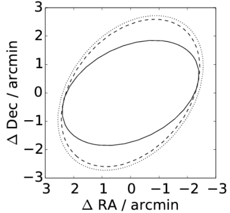
Figure 6.: An exaggerated example of the corrections made to the PSF: the solid black ellipse shows a 150 MHz synthesised beam at the zenith; the dashed line shows the synthesised beam for a pointing due South, at a zenith angle of 45^\circ ( 15^\circ further than the maximum zenith angle of MWACS), resulting in a stretch in Dec; the dotted line shows an increase in the size of the PSF by a further 5%; the real magnitude of the correction is closer to 2%, and accounts for the effects of ionospheric smearing and image-based mosaicking.
