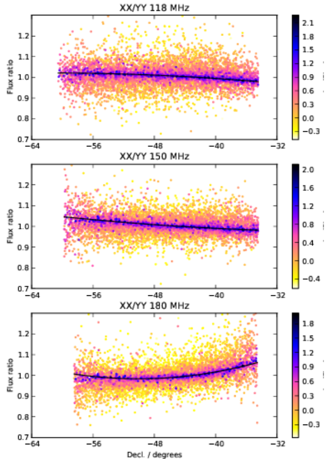
Figure 10.: Ratio of XX to YY flux density for all sources detected in both maps plotted against Dec for all frequencies (low to high). The colour axis is the \log_{10} of the source flux density in Jy (as measured in the YY scan before amplitude calibration).
