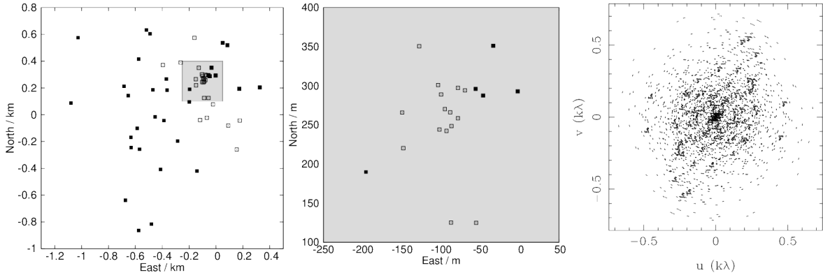
Figure 1.: The left and middle panels show the antenna layout of beta (empty squares) and gamma (filled squares). The light gray shaded box on the left panel is enlarged in the middle panel, to more clearly display the central tiles. The monochromatic zenith-pointed snapshot combined u, v -coverage of the two MWA sub-arrays at 150 MHz is shown on the right.
