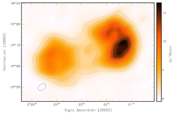
Figure 18.: Fornax A at 180 MHz; contours are linear at 10% levels from the peak brightness of 16.75 \text{ Jy beam}^{-1} . The synthesised beam is shown as an open ellipse at the bottom-left of the image, with dimensions 4'.22 \times 2'.85 , position angle -53.8 . The RMS of this image is 92 \text{ mJy} .
