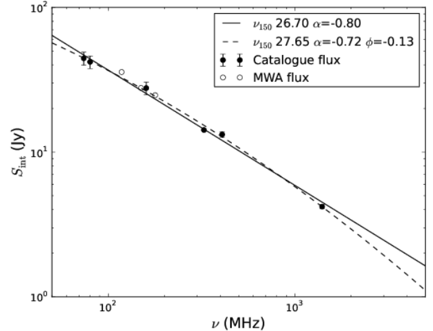
Figure 8.: 3C32 flux densities from the VLSS, Culgoora, MRC, and NVSS surveys shown with uncorrected MWA fluxes. Two fits to the non-MWA points are shown: the solid line is a power-law (i.e. a straight-line fit in log-log space); the dashed line fits a parabola in log-log space. MWA flux densities were corrected to lie on the power-law fit.
