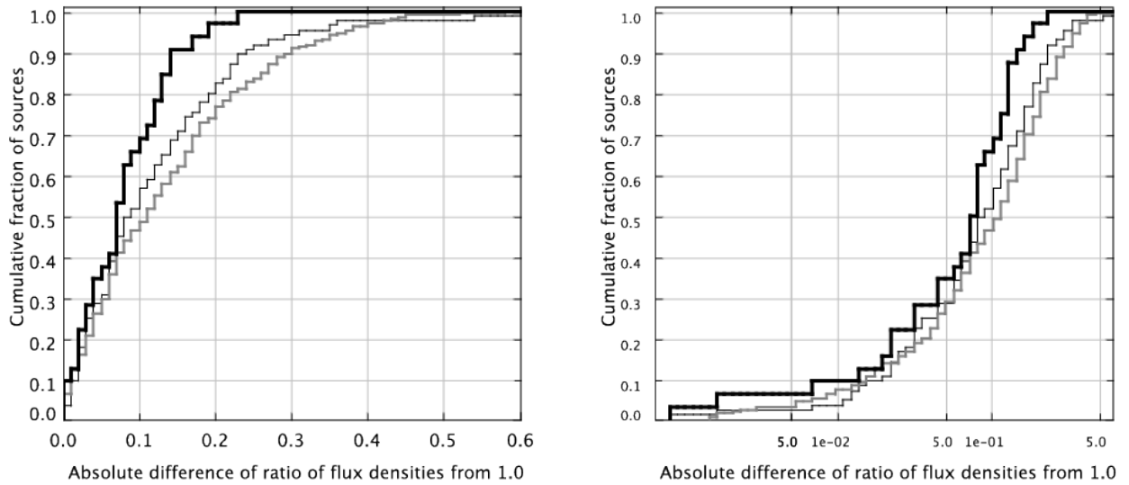
Figure 12.: The cumulative histograms of the difference of the flux density ratio from unity, where the ratio is the ratio of the flux densities of unresolved sources found in MWACS to the flux densities as measured by other catalogues (see Section 3.9.1). The grey line shows Culgoora, the thin black line shows all MS4 and MRC4 sources, and the thick black line shows only those MS4 and MRC4 sources which do not have curved spectra and are not pure extrapolations from 408 MHz downward. The left panel shows the histogram in linear intervals, while the right panel shows the histogram with a log scale.
