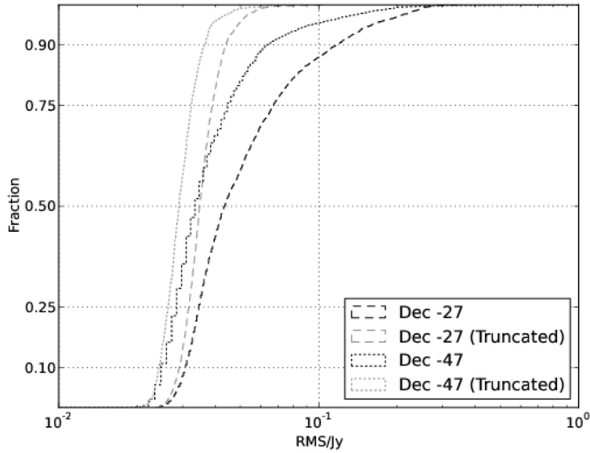
Figure 16.: Cumulative distribution functions of the RMS at 180 MHz for those areas of the map outside of the overlap region for the Dec -27 scan (black dashed line) and Dec -47 scan (black dotted line). A subset of data truncated in RA and Dec range is also shown for both scans: Dec -27 (grey dashed line: 22^{\text{h}}00^{\text{m}} < \alpha < 07^{\text{h}}30^{\text{m}} , -30^{\circ} < \delta < -20^{\circ} ); Dec -47 (grey dotted line: 21^{\text{h}}15^{\text{m}} < \alpha < 06^{\text{h}}40^{\text{m}} , -42^{\circ} < \delta < -52^{\circ} )
