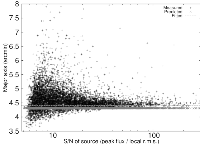
Figure 5.: An example of the analysis used to find the correct PSF for the mosaicked images: in this case, we examine the major axis of sources detected in the zenith scan at 180 MHz. The black crosses show the measured major axis of each source against its signal-to-noise ratio (S/N); the grey stars show the expected major axis if the zenith-angle-dependent projection effect were the only source of change in the synthesised beam; the light grey dashed line shows a S/N-weighted horizontal fit to the major axis measurements. The ratio of this fit to the predicted major axis gives the correction factor by which the major axis of the PSF must be increased to match the data: see Table 2 for a list of the corrected PSFs for each mosaic.
